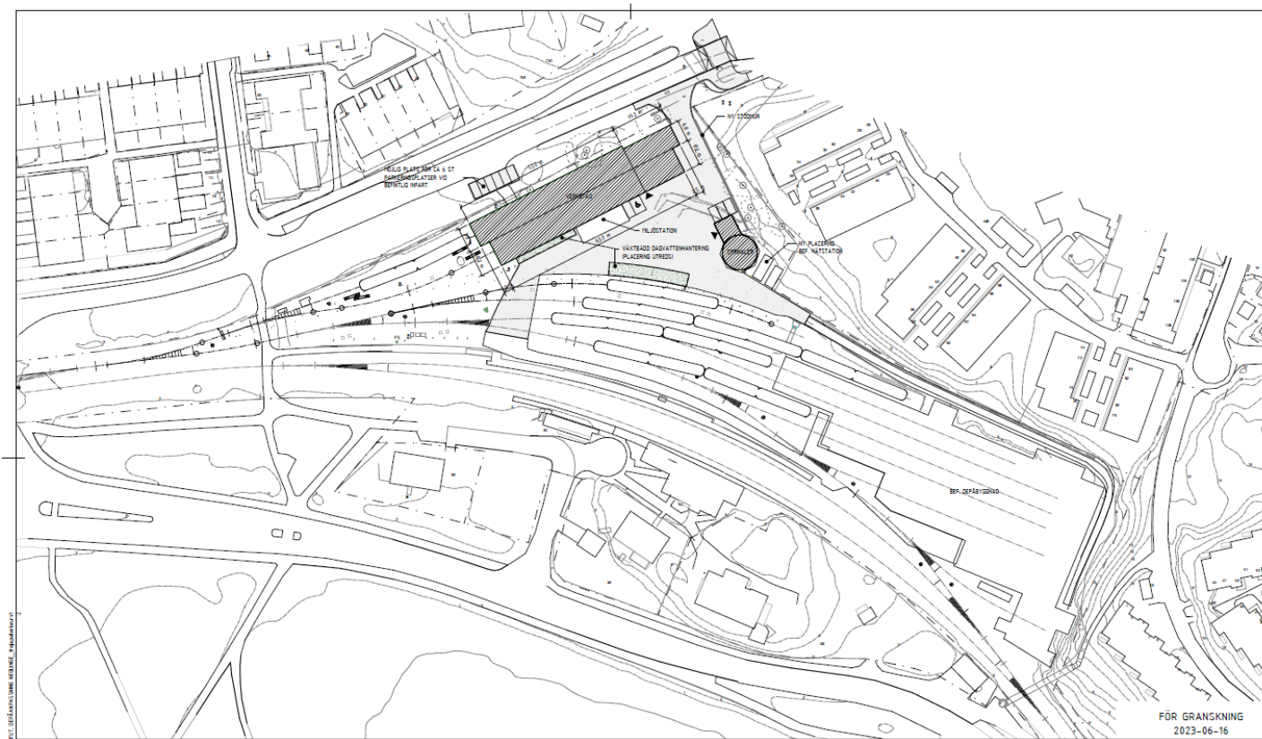
Figur 23. Situationsplan. Programhandling 2023-06-16
